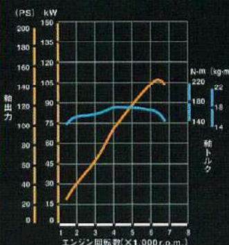
BEAMS 1ZZ-FE VVT-i Displacement: 1,794cc Maximum Power: NET107kW (145PS) / 6,400r.p.m. Maximum Torque: NET171N·m (17.4kg·m) / 4,200r.p.m.
